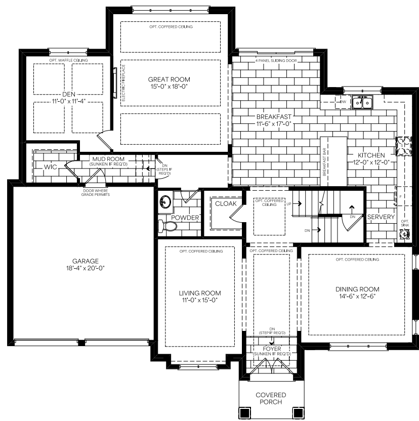
Main Floor Elevation A
