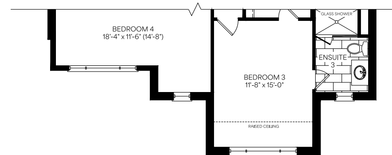
Second Floor Elevation C
