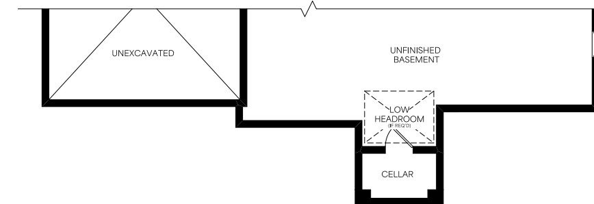
Basement Elevation C
