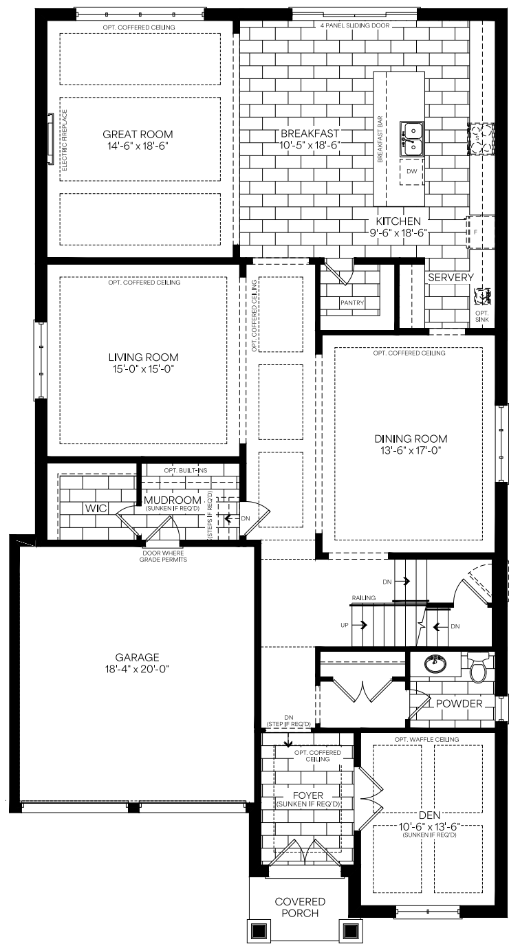
Main Floor Elevation A
