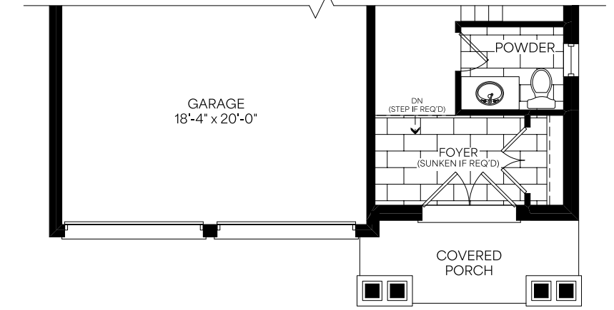
Main Floor Elevation B
