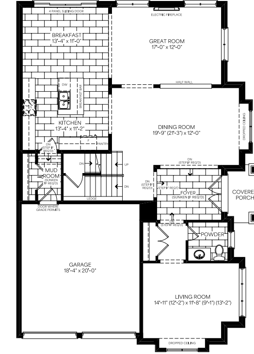
Main Floor Elevation A2
